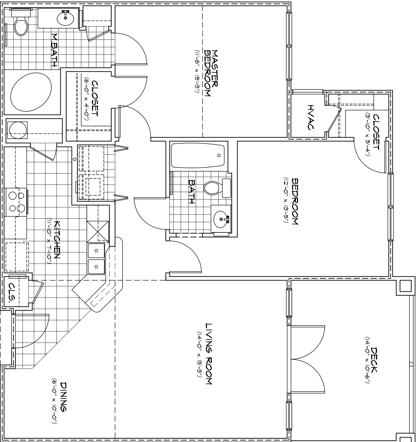
TWO BEDROOM DECK UNIT
